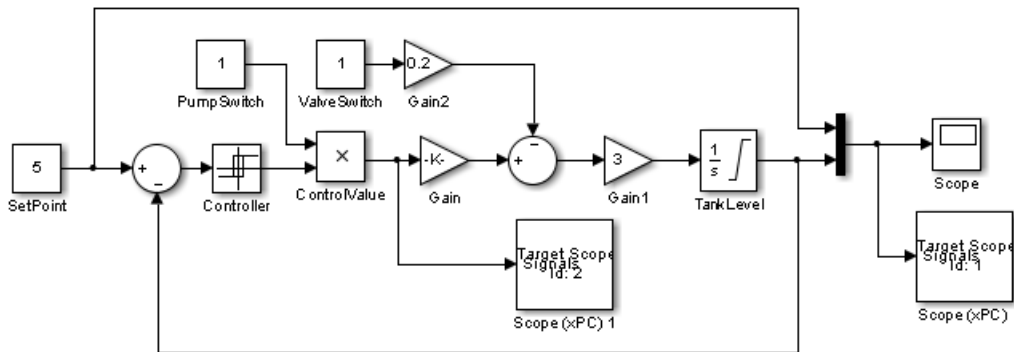
Tank Level Control System
